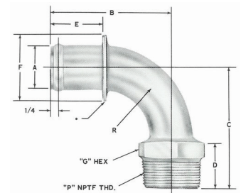
23871 90° Elbow NPTF Male Thread
