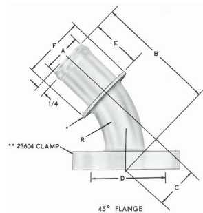
23868 45° Elbow S.A.E. Flanged Head
