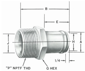
20350 Straight NPTF Male Thread
