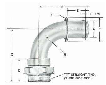
23869 90° Elbow Male O-Ring Seal
