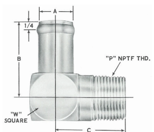
23916 90° Elbow NPTF Male Thread
