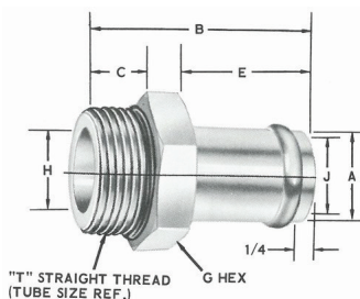
23540 Straight S.A.E. Straight Head
