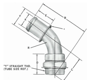
23870 45° Elbow Male O-Ring Seal
