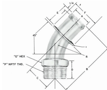
23872 45° Elbow NPTF Male Thread
