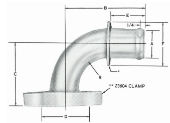
23867 90° Elbow S.A.E. Flanged Head
